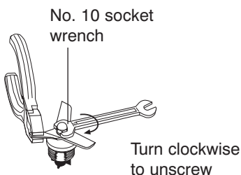
Disassembling blade
